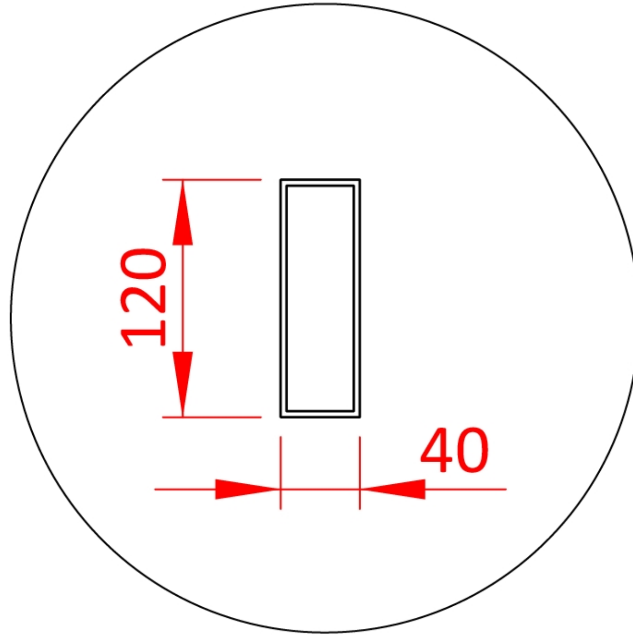
Cross Beam
