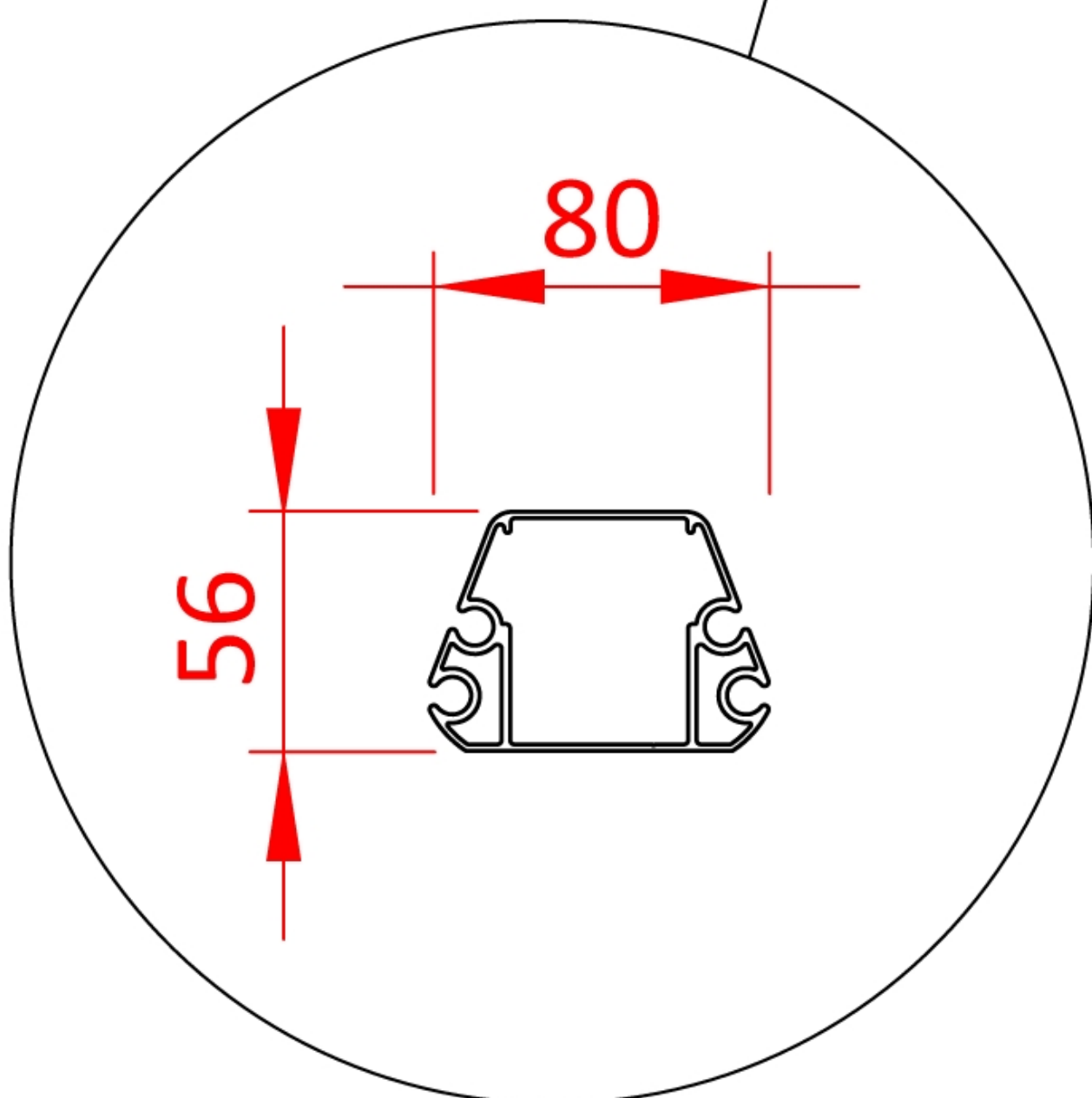
Fabric Support Profile (Double)
