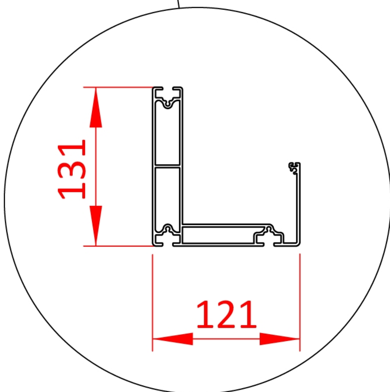
Gutter Profile
