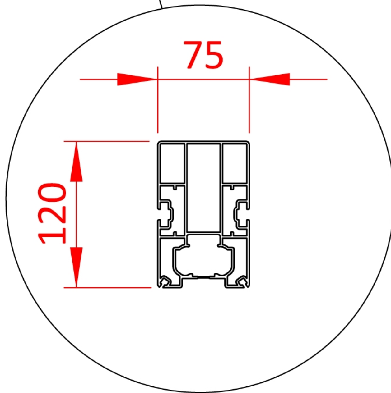
Rail Profile
