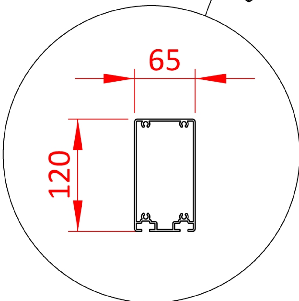
Front Pillar
